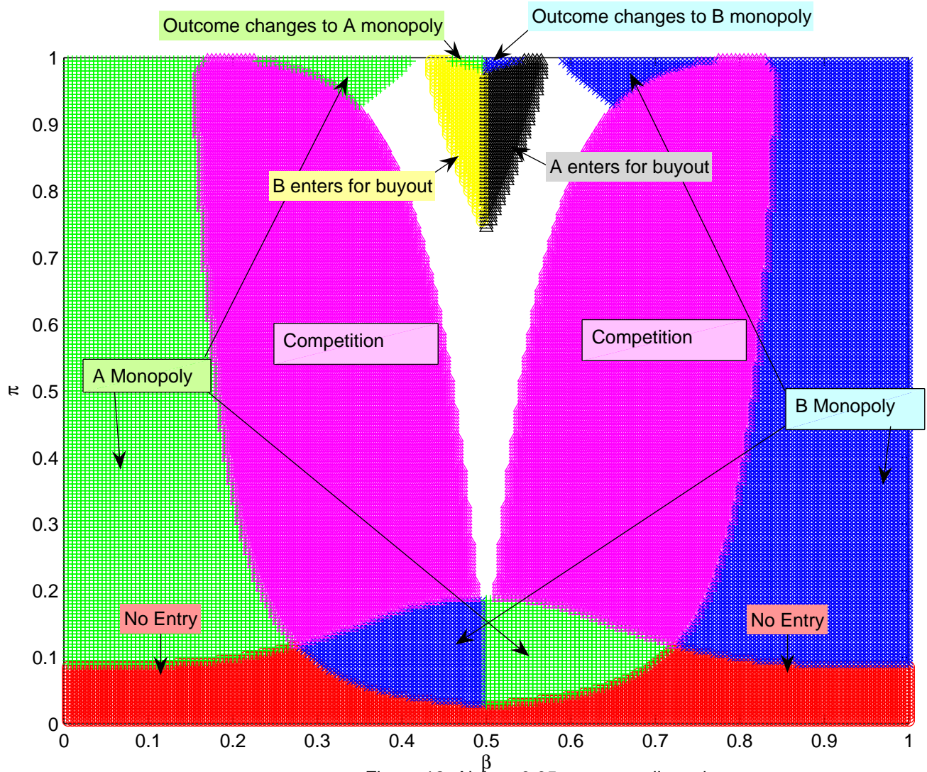
Figure 12: Alpha= 0.05, mergers allowed
